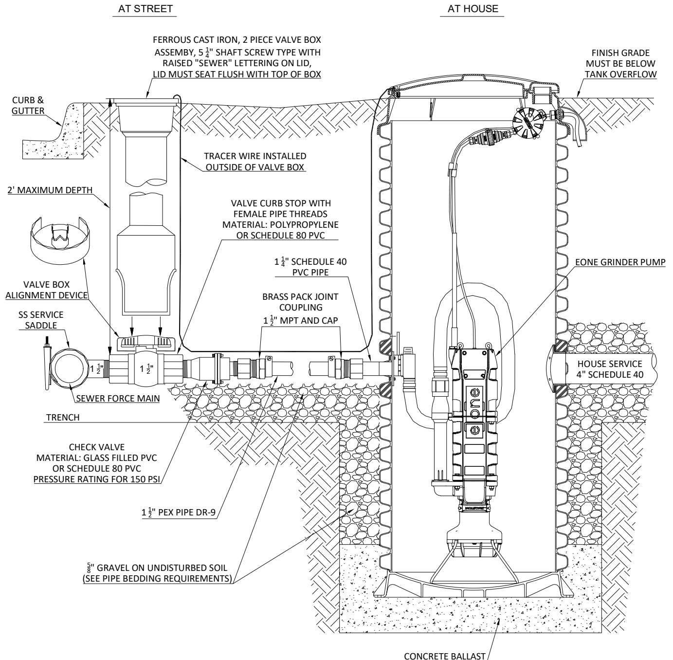
Low Pressure Grinder Pump Service Line Detail
