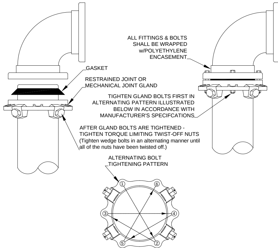
Mechanical Joint & Restrained Joint Connections
