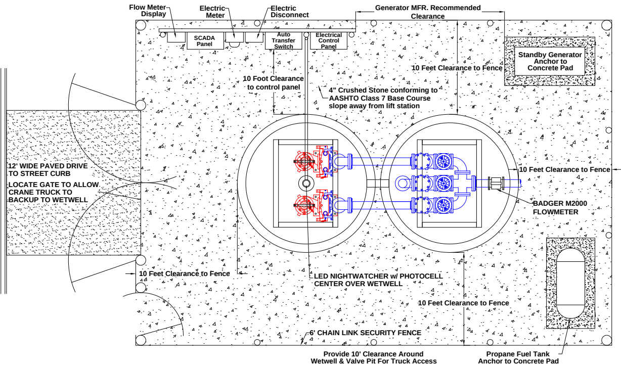
Typical Lift Station Plan View
