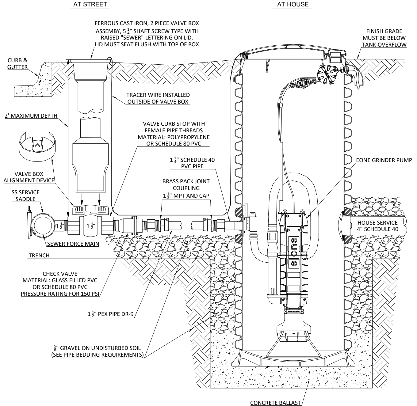
Installation Detail
