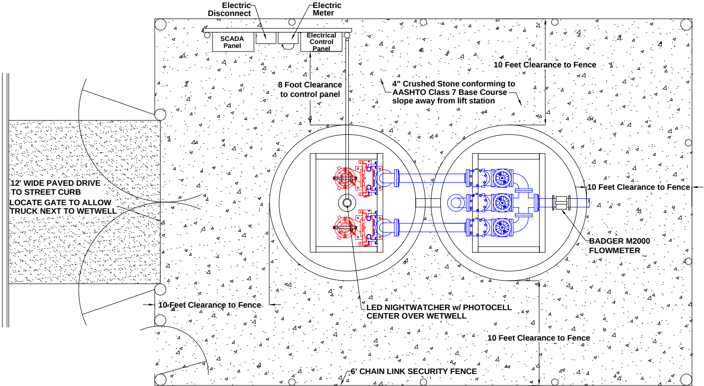
Typical Lift Station Plan View
